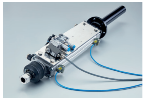
RETRACTION SYSTEMS FOR IGNITERS/FURNACE CAMERAS
